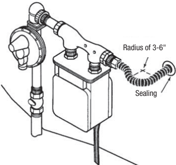
Figure 4.14 Independently Supported Meter
